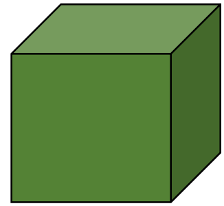
Kube
