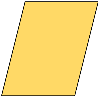
Parallelogram
